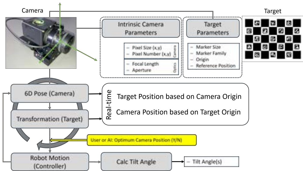
Figure 3: Scheme of a typical calibration process using a ChAruCo target and an imaging system (camera with lens) with known intrinsic parameters
