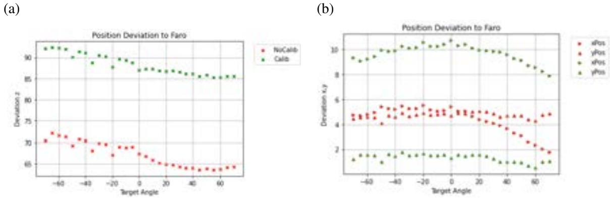
Figure 10: Position deviation: green is Calib, red NoCalib (a) z position, (b) x, y position
