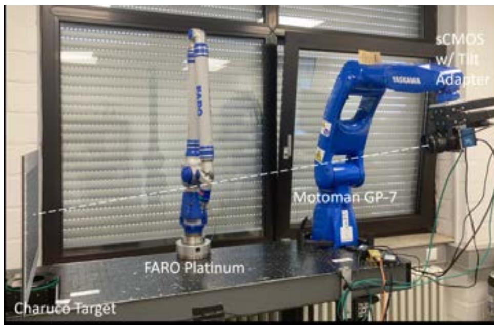
Figure 5: sCMOS camera mounted on GP-7 robot arm rotated around x and y axis, pointing towards the center of the ChArUco target plate. FARO measuring arm was used as position reference.
