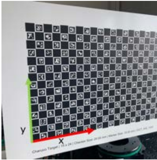
Figure 1: Calibration checkerboard (a) ( ChArUco ) with ArUcoTag bundle. (b) detail showing individual ArUco tags of type DICT_5x5_1000 each with 5 \times 5 bit encoding.
